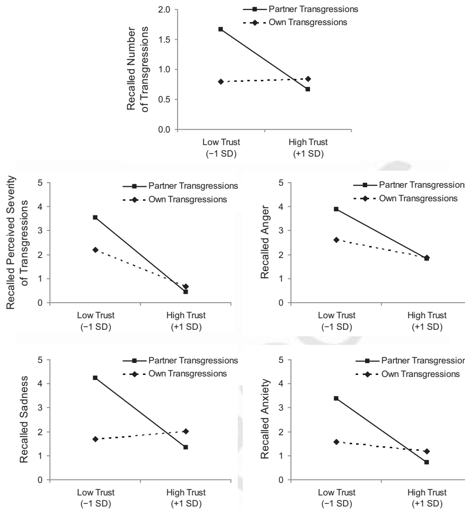
Figure 1. Study 4, from trust and actor (partner vs. self): A. Predicting recalled number of transgressions. B. Recalled perceived severity of transgressions. C. Recalled anger. D. Recalled sadness. E. Recalled anxiety. Each panel presents model implied levels of the memory criterion controlling for the mean value of the corresponding initial report. The memory criteria presented in Panels B–E were assessed on a 0–6 scale.
