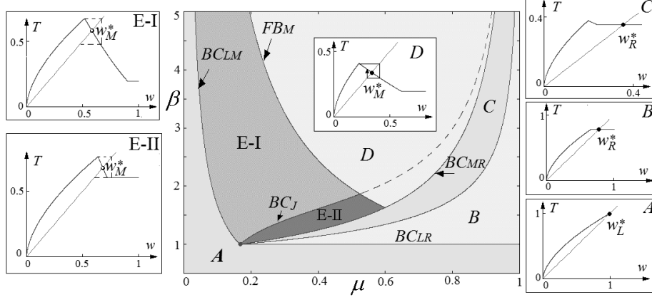
Figure 1: Basic bifurcation curves of map T in (\mu, \beta) -parameter plane at m = 1.2 , \alpha = 0.6 . Examples of map T in different parameter regions are also shown.
