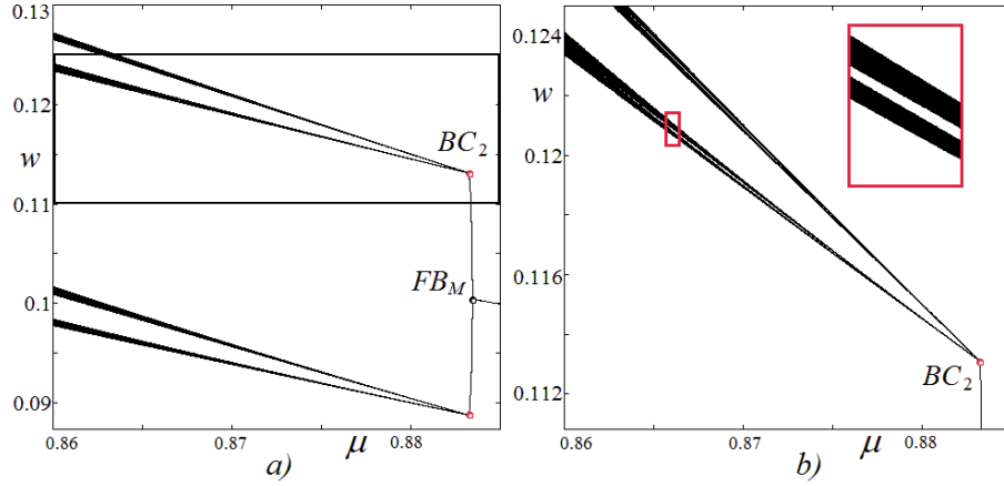
Figure 4: 1D bifurcation diagram in the map T for \alpha = 0.9, m = 1.005, \beta = 1.315, \mu \in [0.86, 0.885] is shown in a) , and its enlargements are in b) . Here the BCB of the 2-cycle leads to 8-cyclic chaotic intervals.
