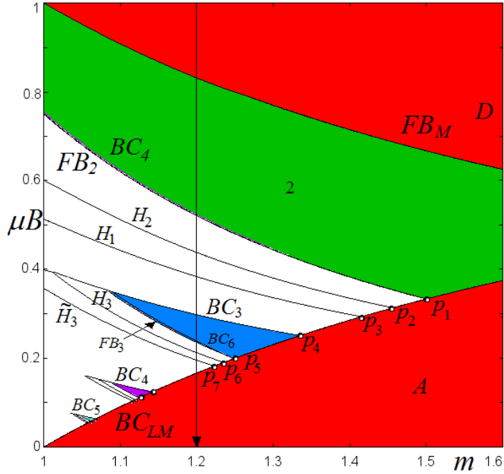
Figure 6: 2D bifurcation diagram in the (m, \mu B) -parameter plane at \alpha = 0.5 . 1D bifurcation diagram at m = 1.2 and its enlargements are shown in Fig.8 and Fig.9.
