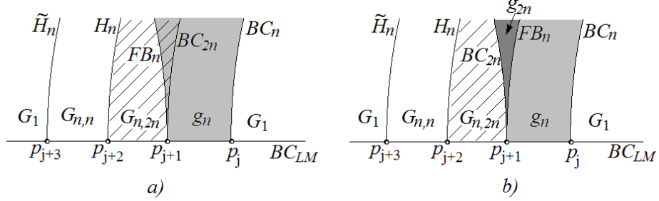
Figure 5: A neighborhood of the curve BC_{LM} shown schematically in case when the BCB curve \mathcal{B}_m given in (24) related to BC_{LM} crosses an n -periodicity region of the skew tent map. The flip bifurcation at FB_n is subcritical in a ) and supercritical in b ). The point p_{j+1} is a border-flip codimension-two bifurcation point.
