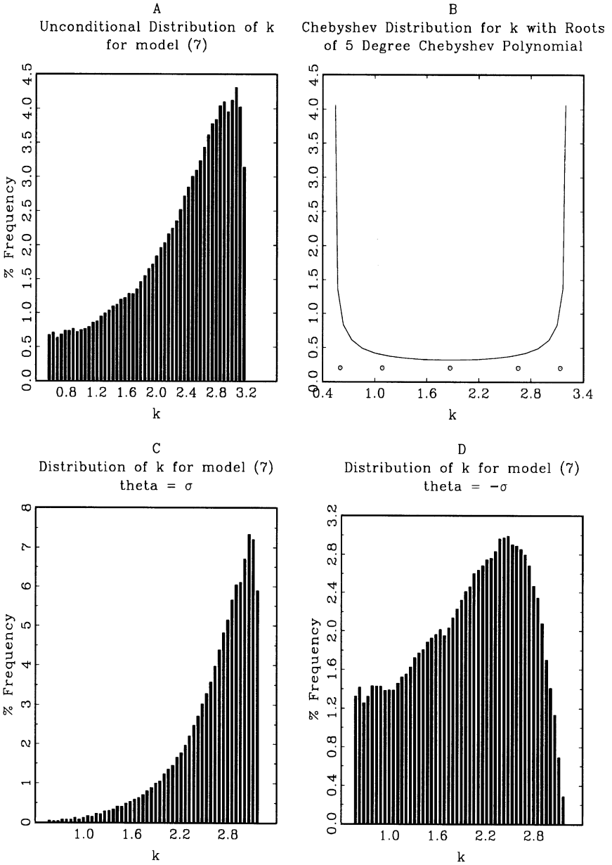
Fig. 5. Endogenous and exogenous capital stock distributions.
