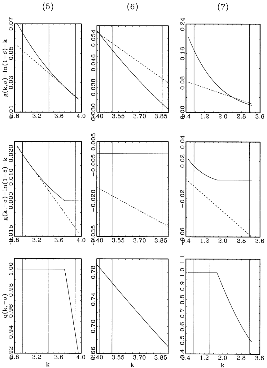
Fig. 3. Policy functions for models (5)–(7). Note: See the notes to Fig 2.
