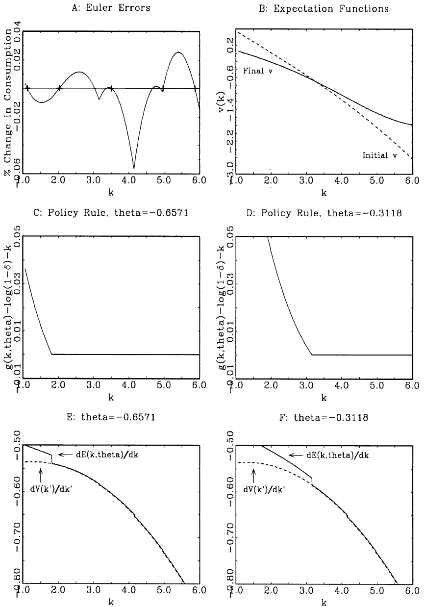
Fig. 7. PEA collocation with the Wright-Williams conditional expectation.
