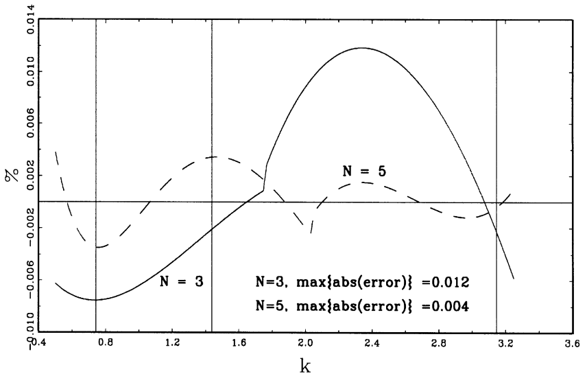
Fig. 6. Euler errors for PEA collocation on model (7).
