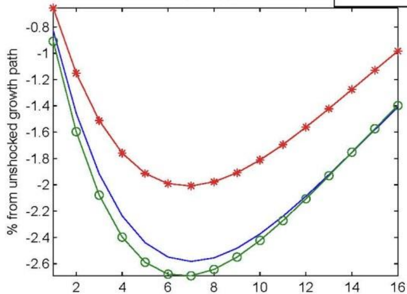
C: investment
