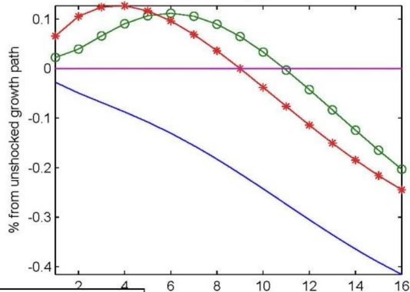
B: consumption
