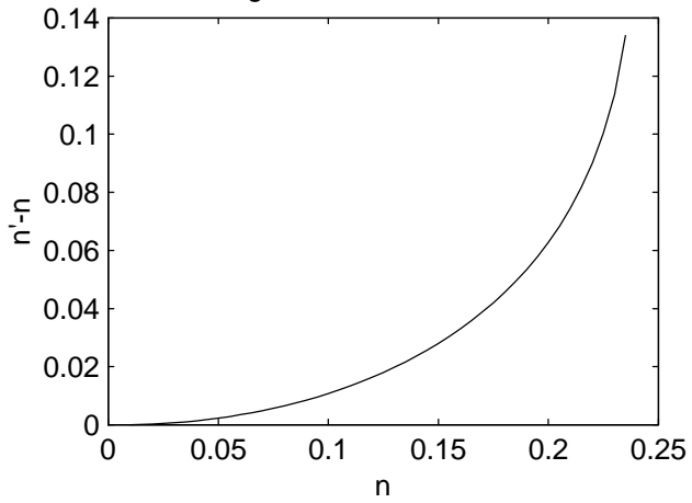
Figure 6c: n' - n versus n
