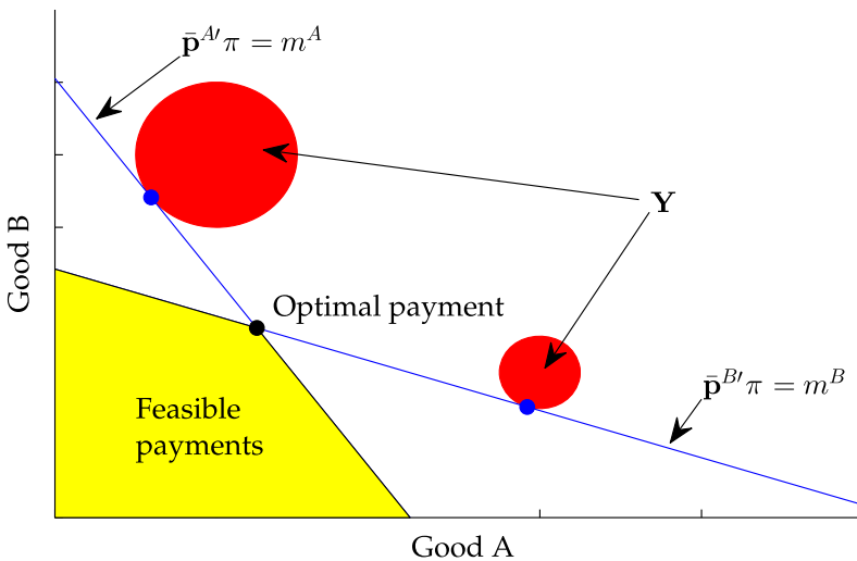
FIGURE 1.—Determination of optimal unit of account.
