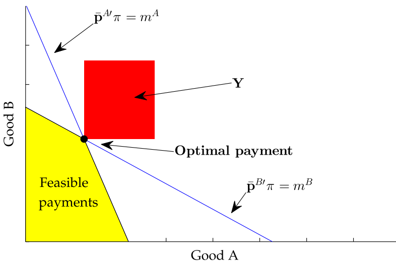
FIGURE 2.—Determination of optimal unit of account with rectangular endowment set Y .
