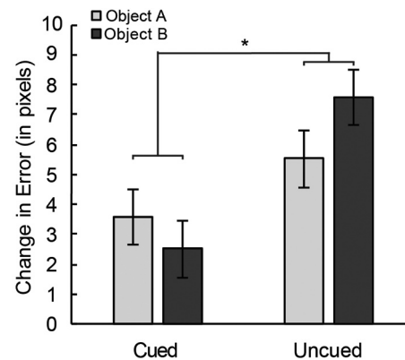
Fig. 2. There was less forgetting from the pre-nap test to the post-nap test for object locations cued during sleep than for those not cued. This cueing benefit was not significantly different between Objects A and B. Error bars reflect \pm 1 standard error of the mean (SEM) for each condition, adjusted to represent the variance for statistically evaluating the cueing benefit, a within-subjects contrast (i.e., SEM was calculated using each participant's value for each condition after subtracting that participant's mean value across all conditions). * - p < 0.05 .
