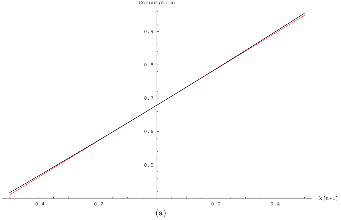
FIGURE 1: CONSUMPTION IN THE STOCHASTIC GROWTH MODEL, c_t(k_{t-1}) FIRST- THROUGH SEVENTH-ORDER APPROXIMATE SOLUTIONS
