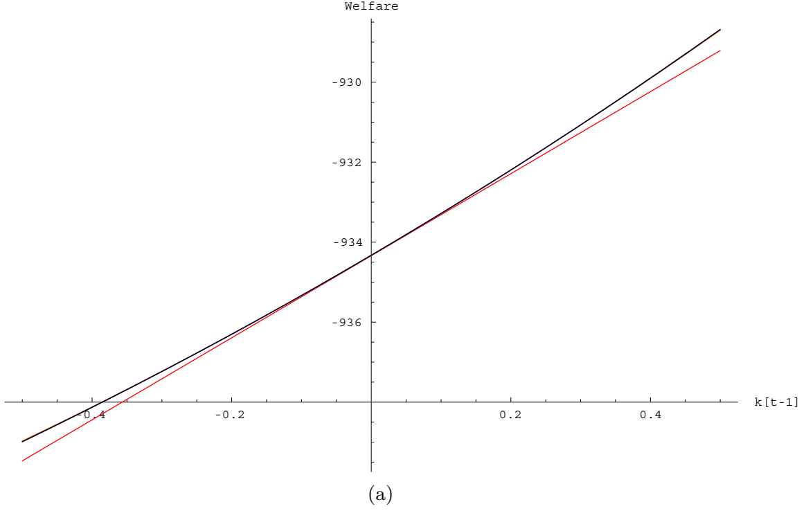
FIGURE 2: WELFARE IN THE STOCHASTIC GROWTH MODEL, \text{Welf}_t(k_{t-1}) FIRST- THROUGH SEVENTH-ORDER APPROXIMATE SOLUTIONS
