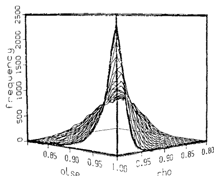
FIGURE 2.—Joint frequency distribution of \hat{\rho} and \rho .
