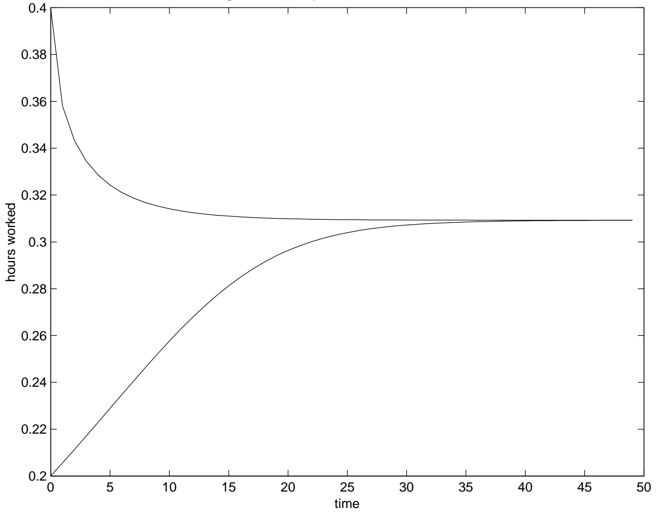
Figure 2: Two Equilibria on the Lower Branch
