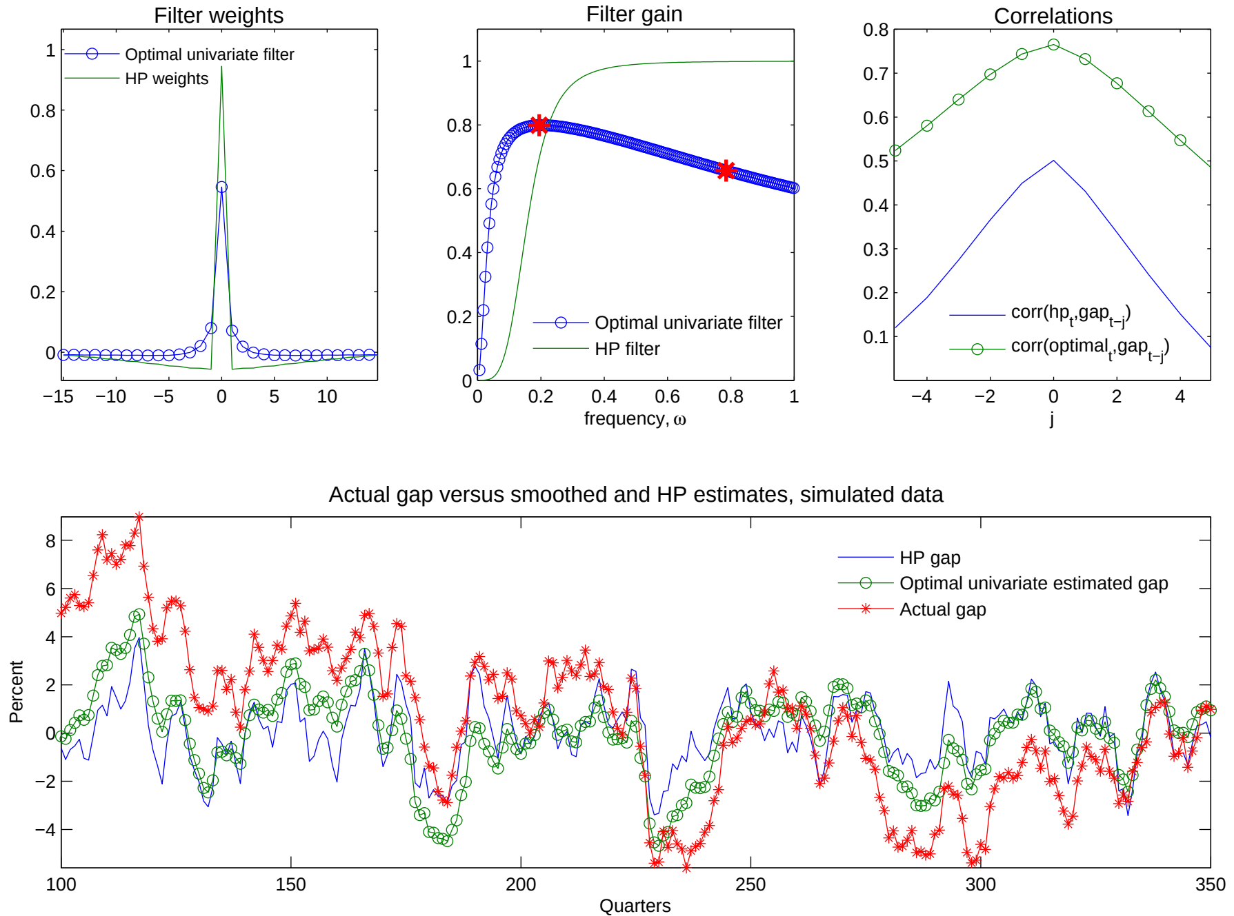
Figure 3: HP Filter and Optimal Univariate Filter for Estimating Output Gap
