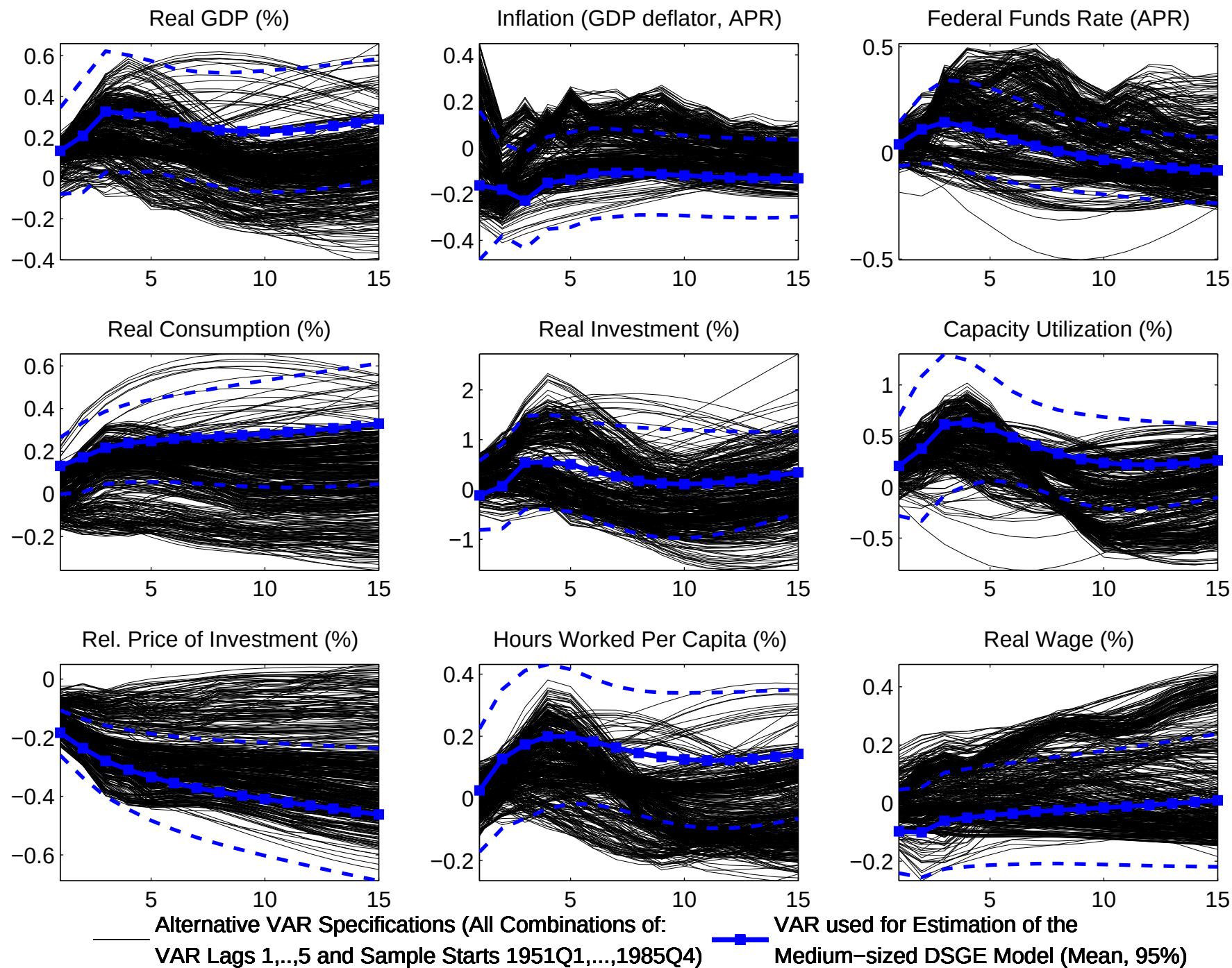
Figure 15: VAR Specification Sensitivity: Investment Specific Technology Shock
