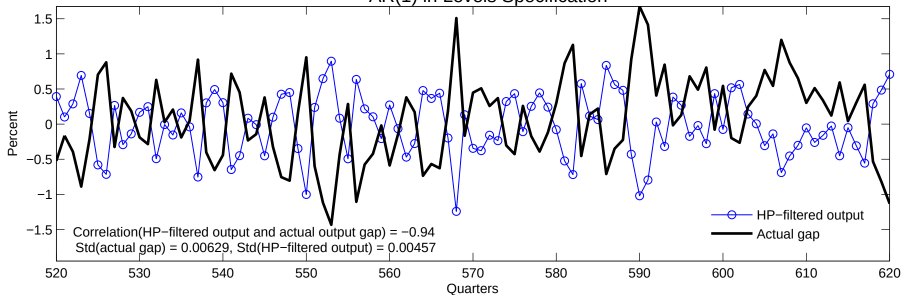
Figure 9b: HP Filter Estimate of Output Gap Versus Actual Gap (Simulated Data) AR(1) in Levels Specification
