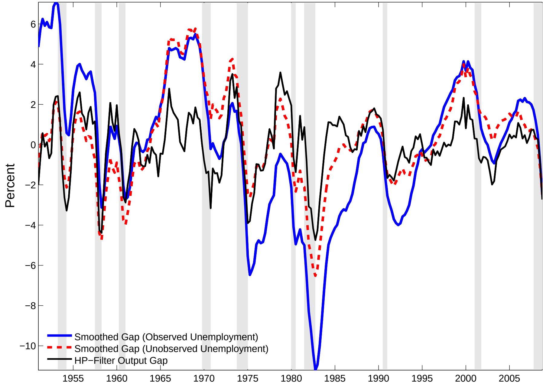
Figure 4: Output Gap in US Data
