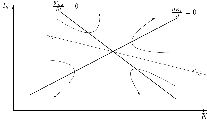
Figure 1: Phase diagram of the economy
