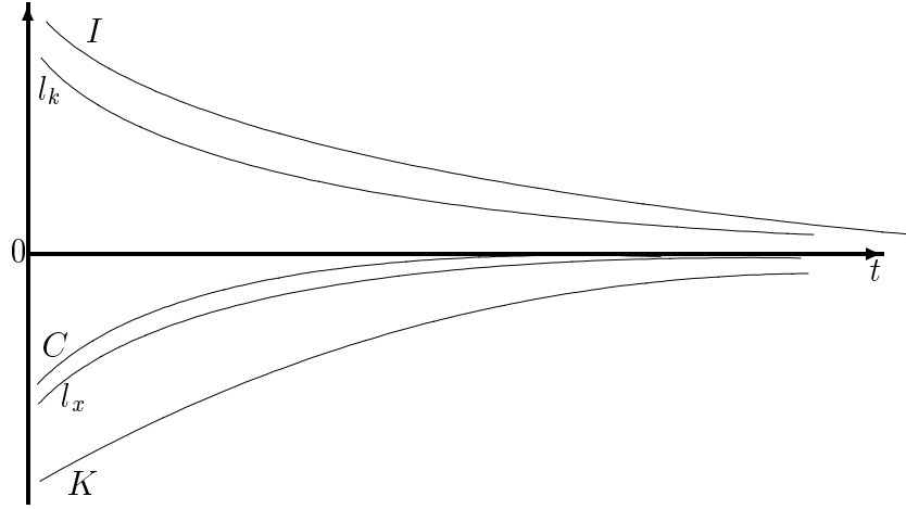
Figure 2: Transitional dynamics with K_0 below steady state (all variables are measured in relative deviations from their respective steady-state level)
