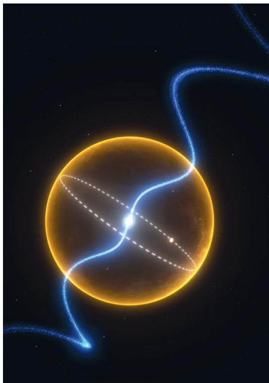
A black widow's companion. Artist's view of PSR J1719–1438 and its planet. The millisecond pulsar is at the center, and the orbit of the planet is shown by the dashed line, with, for comparison, the size of the Sun shown as the yellow sphere.
