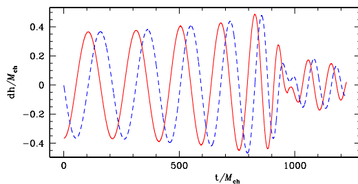
Figure 3. Gravitational wave signal in the h_+ (solid line) and h_\times (dashed line) polarizations, for an observer located at a distance d from the system along the rotation axis. Units are as in figure 2. We see a chirp signal during the inspiral, followed by a lower-amplitude, modulated burst of high-frequency emission while the remnant forms.
