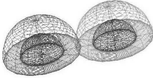
Figure 1. Radial domains used to solve the field equations of the CF method. Each vertex is a collocation point (from [14]).
