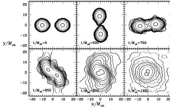
Figure 2. The evolution of the coalescing NS binary. Density contours are logarithmically spaced, two per decade. We see the development of significant tidal lag angles at t/\mathcal{M}_{\text{ch}} = 500 , followed by an ‘off-center’ collision that leads to the formation of a vortex sheet and a small amount of matter ejection, finally resulting in a differentially rotating spheroidal configuration which is stable against gravitational collapse. Units are defined such that G = c = 1 , and \mathcal{M}_{\text{ch}} is the chirp mass of the system.
