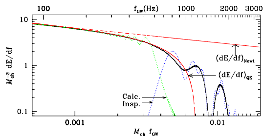
Figure 4. GW energy spectrum, \mathcal{M}_{\text{ch}}^{-2}dE/df , as a function of the GW frequency, \mathcal{M}_{\text{ch}}f_{\text{GW}} . The dotted lines show, respectively at high and low frequencies, the components contributed by our calculated signal and the quasi-equilibrium inspiral component. Also shown are the Newtonian point-mass energy spectrum (short-dashed line), and the quasi-equilibrium fit derived from equilibrium sequence data. On the upper axis, we show the corresponding frequencies in Hz assuming that each NS has an ADM mass M_0 = 1.4M_{\odot} . We see that the ‘break frequency’ occurs well within the sub-kHz regime.
