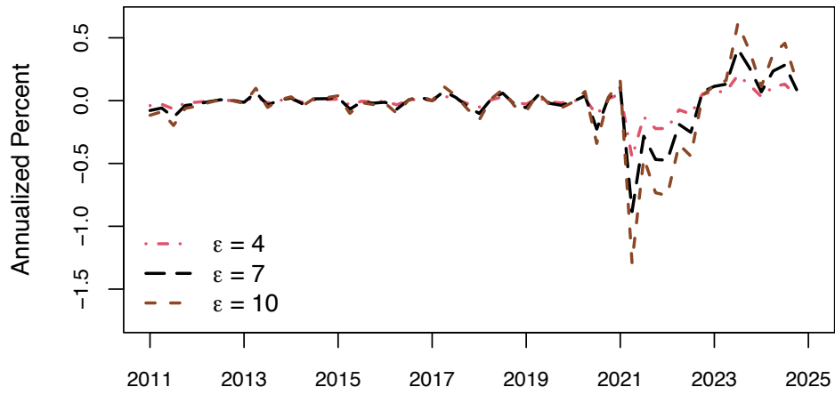
Figure 2: \pi_t^g can be meaningfully different from \pi_t
